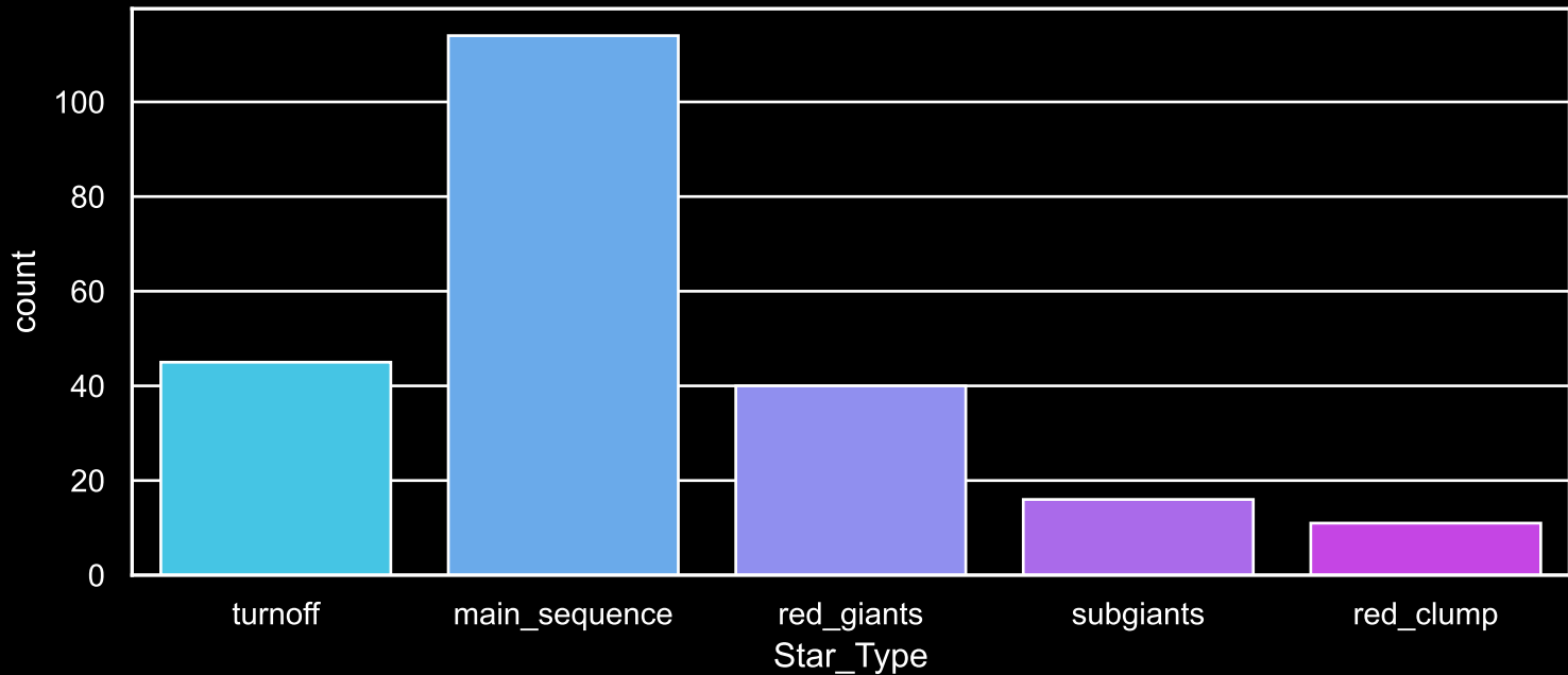
Field [2] Count plot of Star Type
