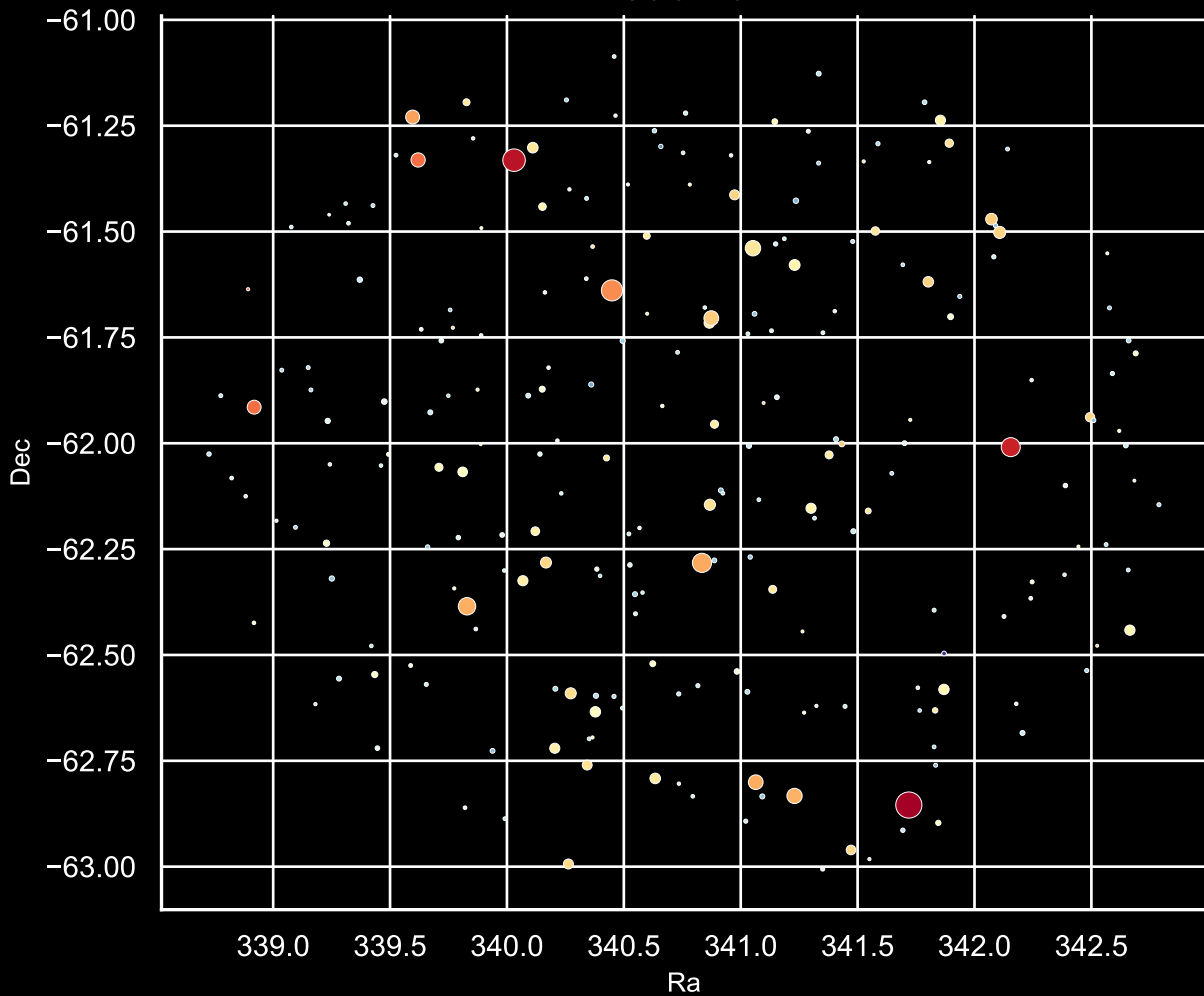
Field [2] Ra [340.77] Dec [-62.03] Stars: 226
