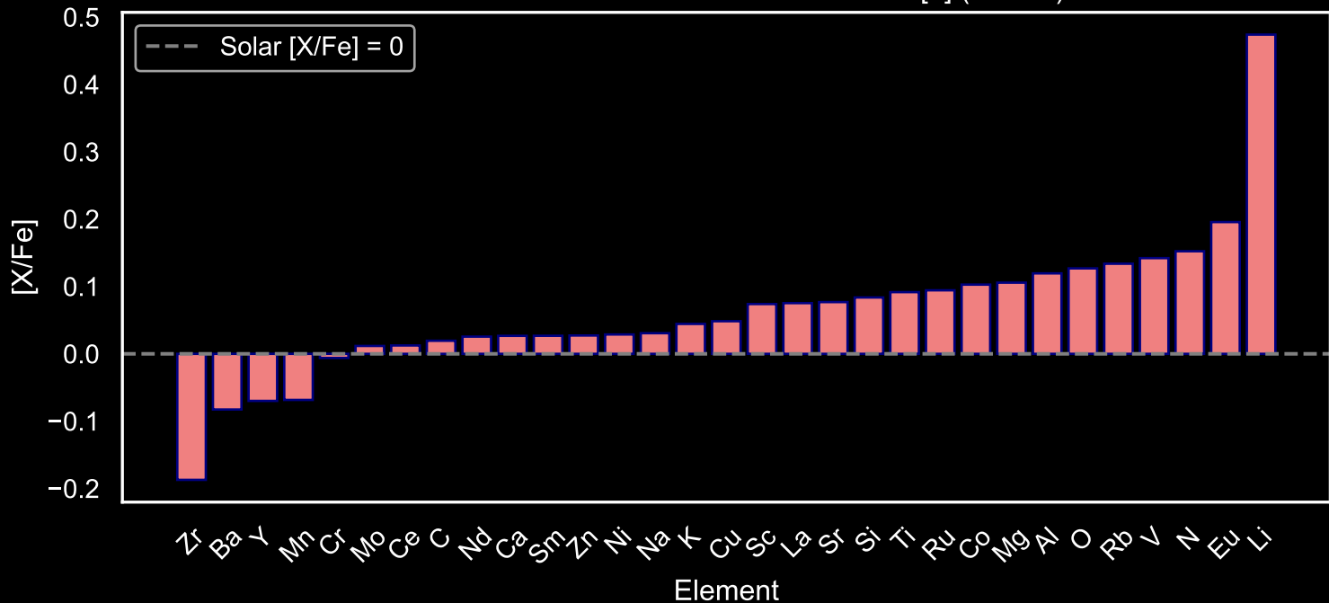
Abundance Pattern for GALAH Star Field [2] (N=226)
