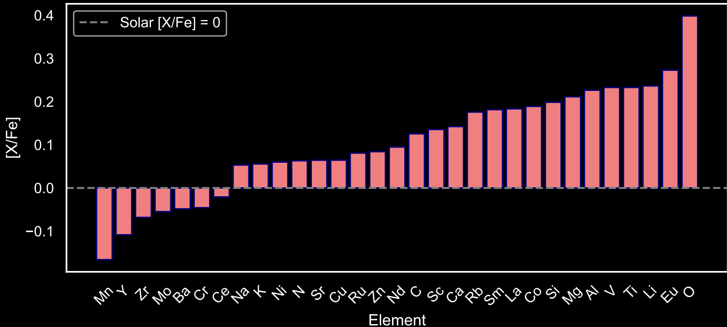
Abundance Pattern for GALAH Red Giants: Star Field [2] (N=51)
