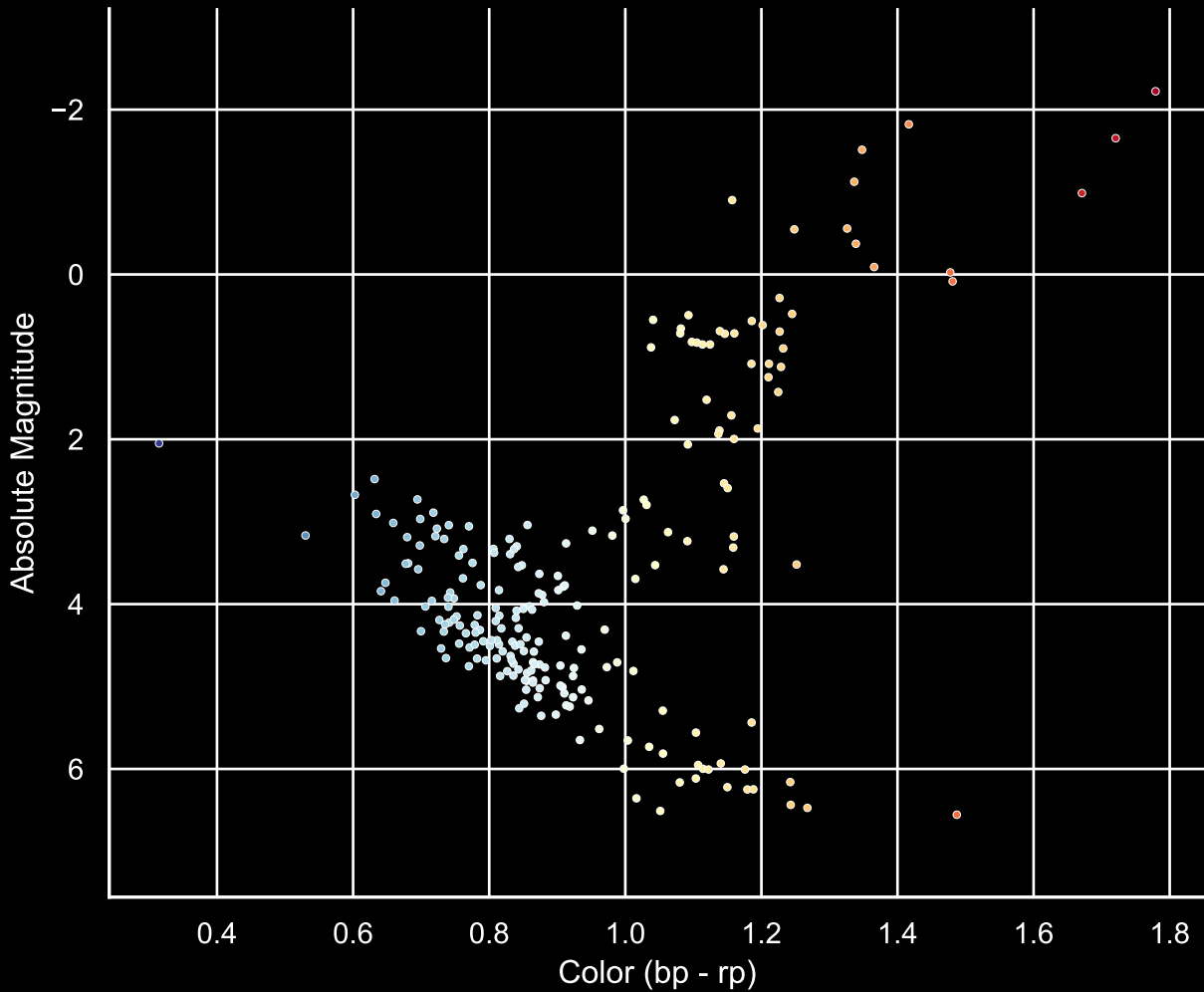
GALAH Hertzprung-Russel Diagram Field [2] Ra [340.77] Dec [-62.03]
