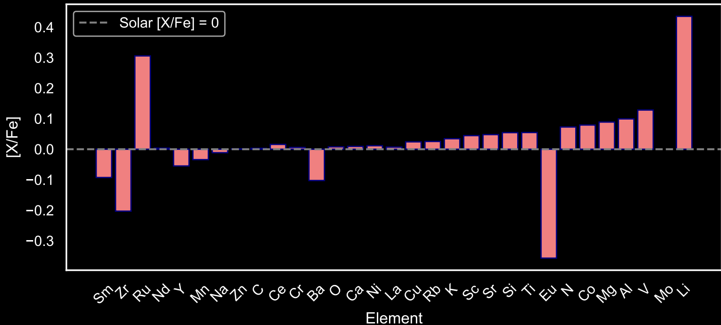
Abundance Pattern for GALAH Main Sequence Stars: Star Field [2] (N=114)
